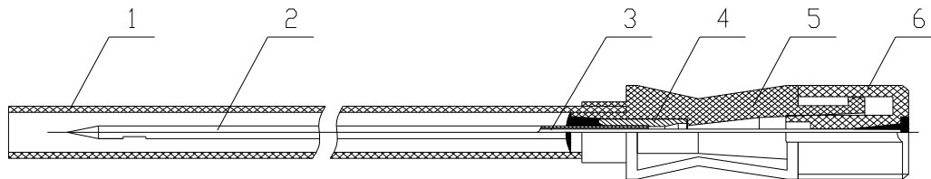
B. representative drawing of KD-FINE spinal needle, Pencil point
