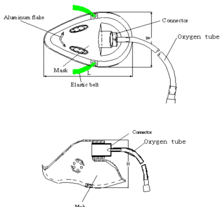
Oxygen Mask
